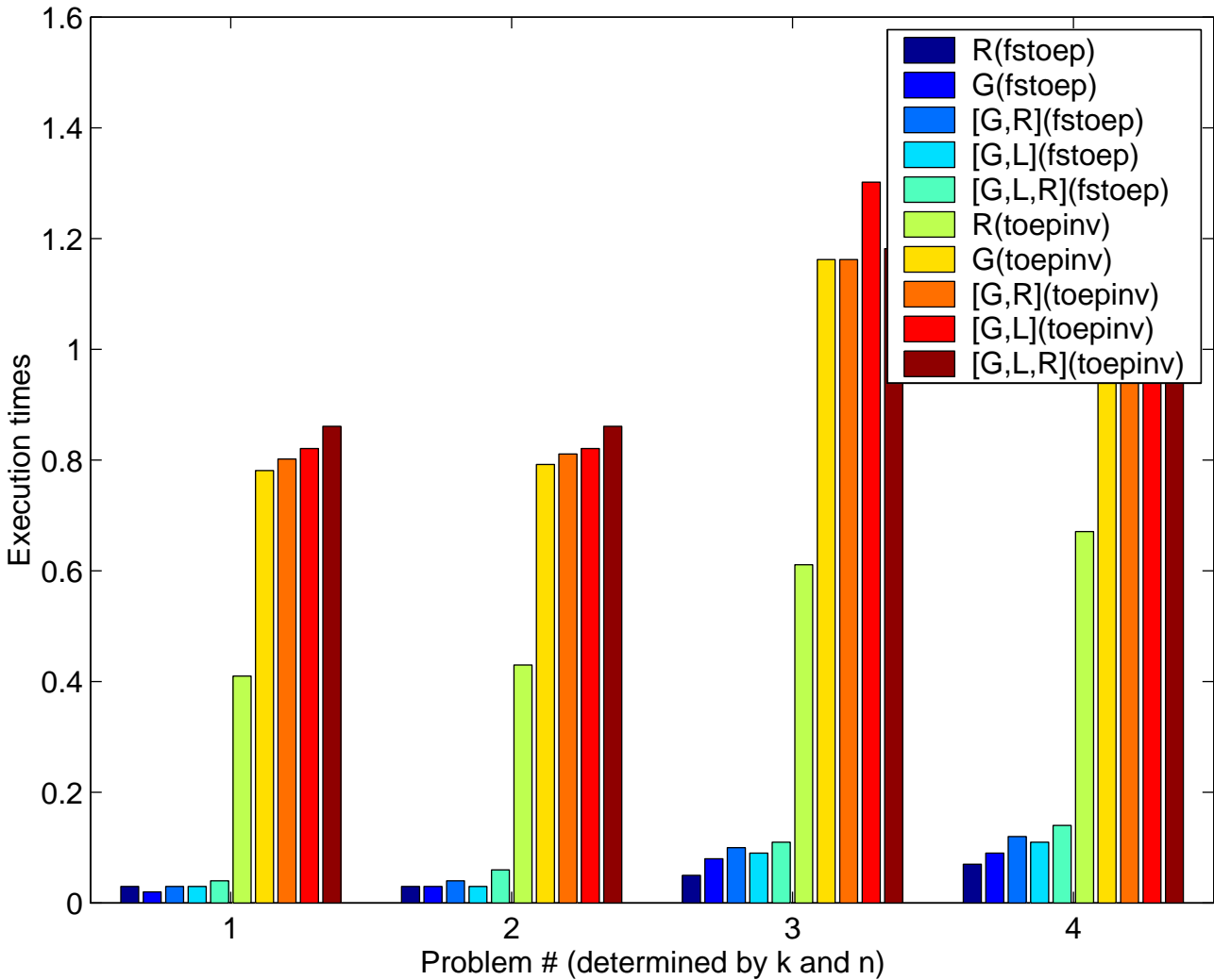
Execution times for factorization
