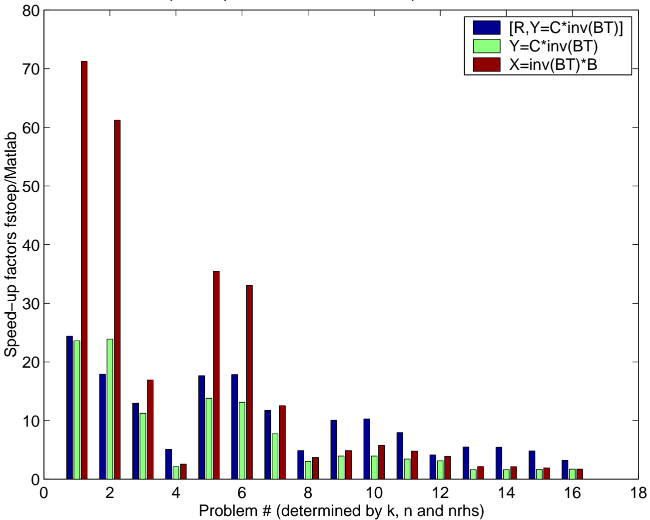
Speed-up factors for solution: fstoep versus Matlab
