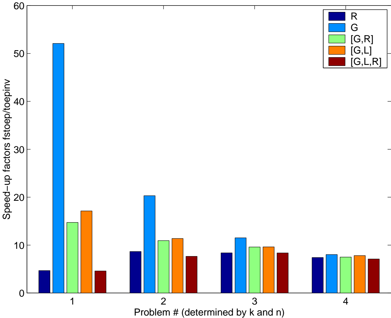
Speed-up factors for factorization: fstoep versus Matlab toepinv
