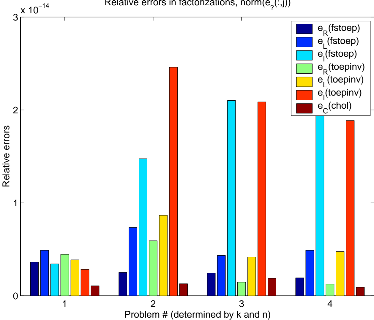
Relative errors in factorizations, \text{norm}(e_\gamma(:,j))
